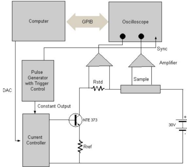
Figure 4.10: Puled measurement setup
