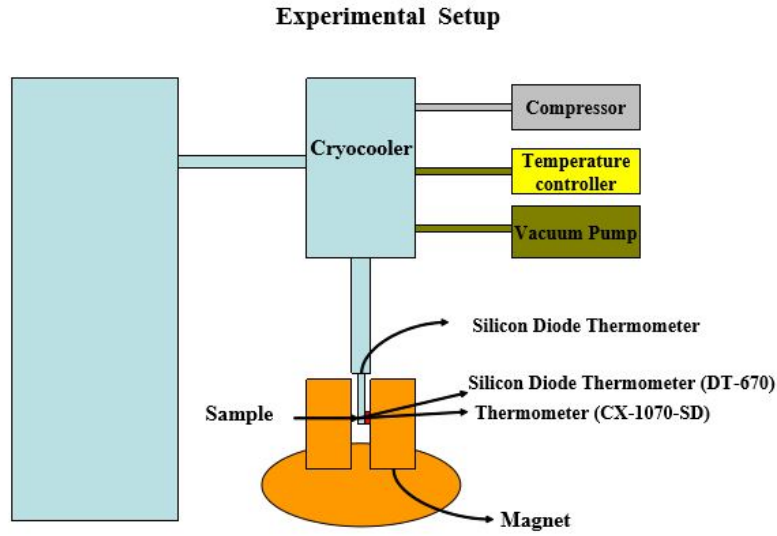
Figure 4.8: Schematic of PT405 and its magnet and sensors
